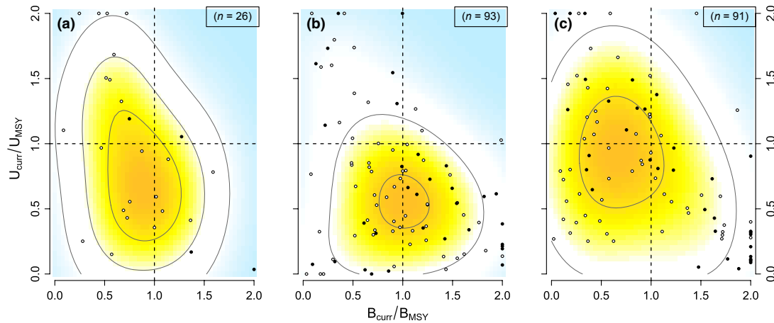
Figure 6 Current exploitation rate vs. current biomass for individual stocks from (a) low ( \geq 2.0 to < 3.0 ), (b) medium ( \geq 3.0 to < 4.0 ) and (c) high ( \geq 4.0 ) trophic levels. Plot details as in Fig. 4.
